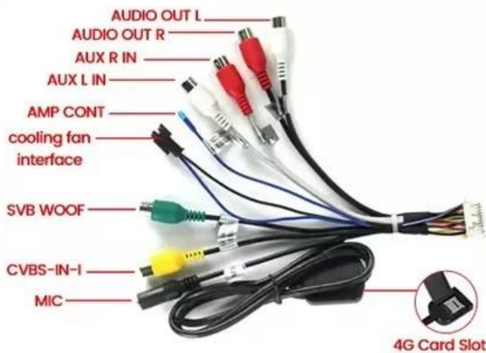
(M200S M400S)
