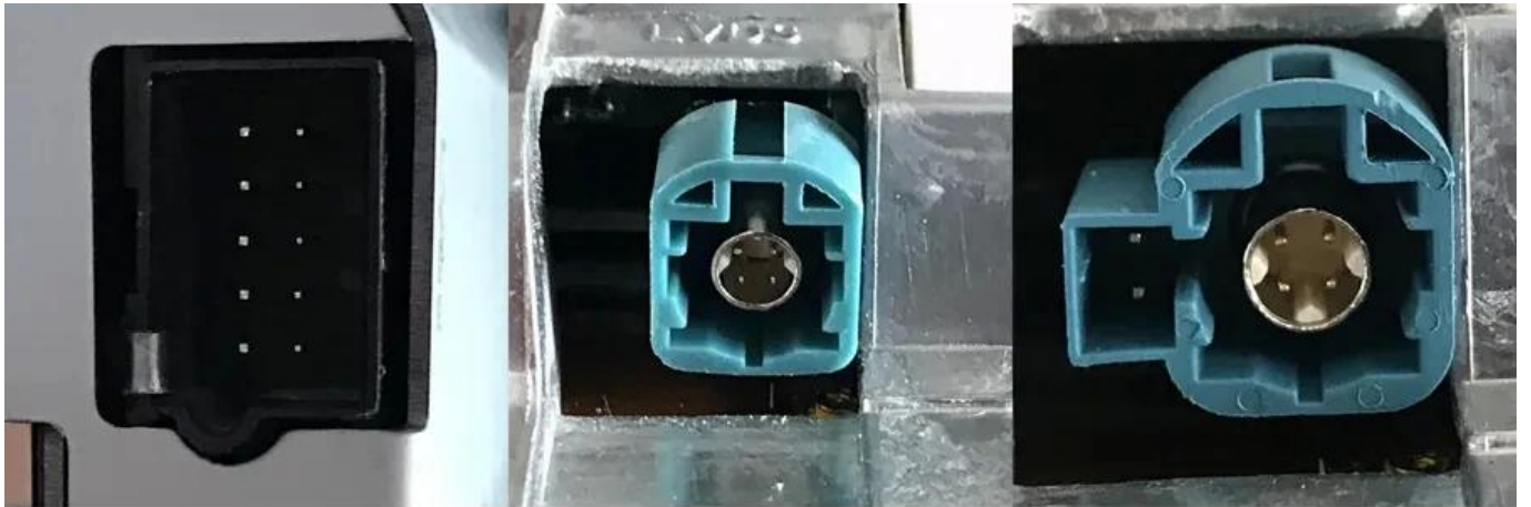
CCC LVDS PLUG (10 pin)
