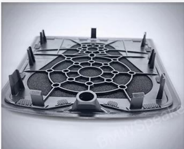
Central perforated cover
